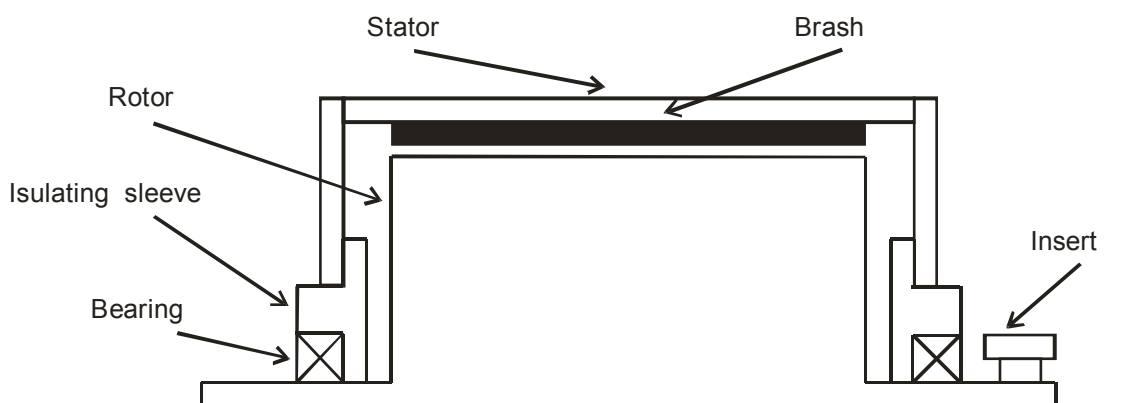
Fig. 5. Generator view in section
