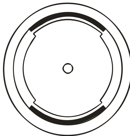
Fig. 4. The electric generator circuit in which the inserts from titanate of barium are located on the internal surface of stator
