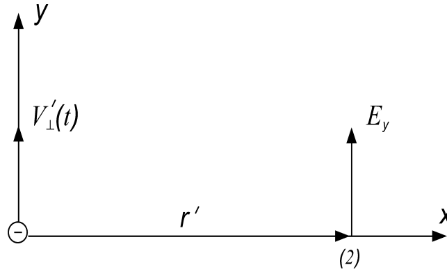
Fig. 4. Formation of the retarded scalar-vector potential.
