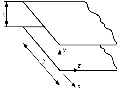
Fig. 5. Two-conductor line consisting of two perfectly conducting planes.
