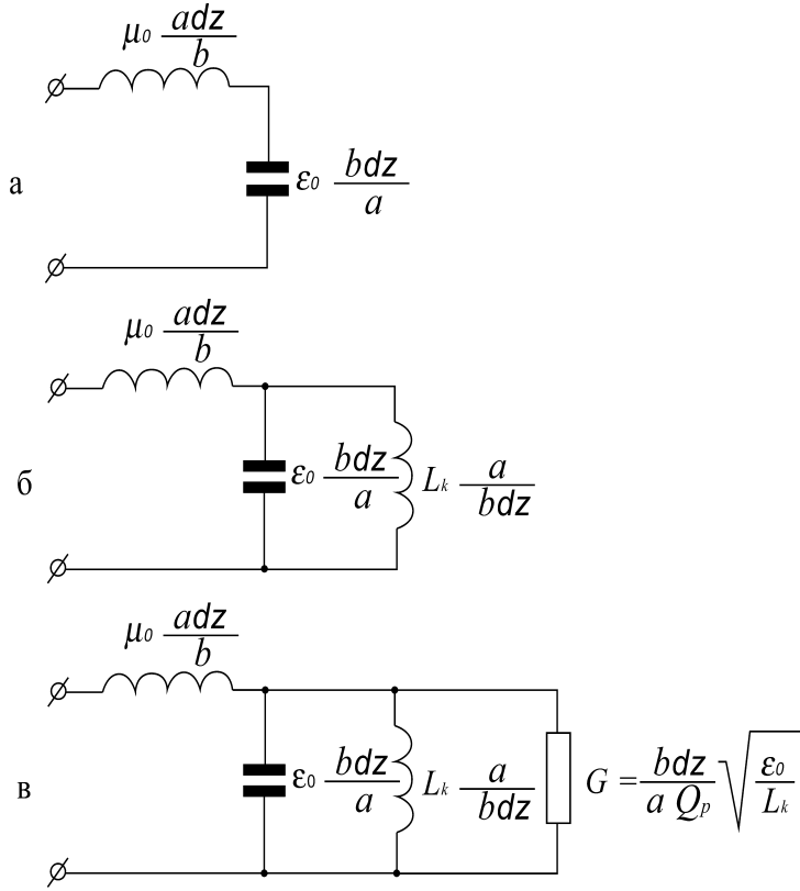
Fig. 6. а. Equivalent circuit of the two-conductor line segment; б. Equivalent circuit of the two-conductor line segment containing nondissipative plasma; в. Equivalent circuit of the two-conductor line segment containing dissipative plasma.
