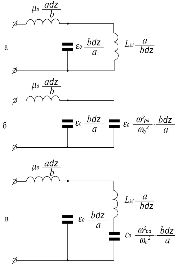
Fig. 7. And б- the equivalent scheme of a piece of the line filled with a dielectric, for a case \omega \gg \omega_0 ; B- the equivalent scheme of a piece of a line for a case \omega \ll \omega_0 .
