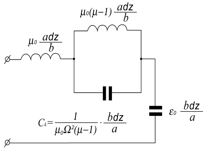
Рис. 8. Equivalent circuit of two-conductor line including a magnet.
