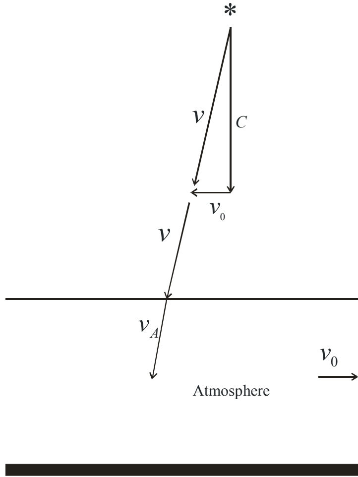
Fig. 3 Diagram of the aberration of light of the star
