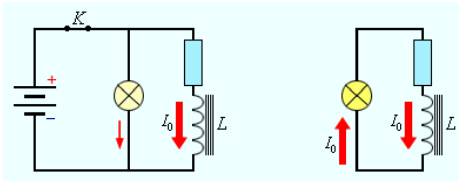
Fig. 6: With closing of key k the lamp vividly flares up
