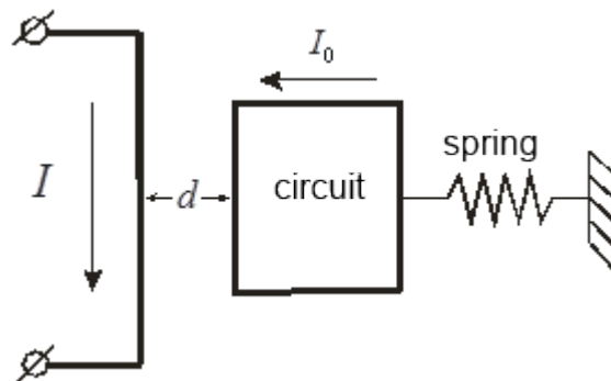
Fig. 7: Outline with the frozen current near the conductor, along which flows the current
