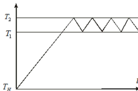
Fig. 24. Temperature graph of cyclic drying regime.
